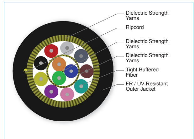
Cross Section of Part Number: 012T8P-31190-29
